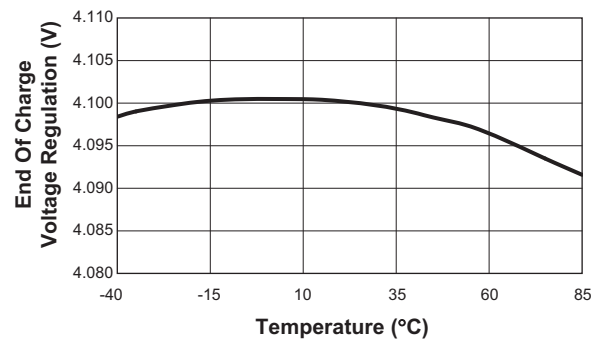
Constant Regulated Output Voltage vs. Temperature (AAT3681A-4.1 and AAT3681A-5 Only)
