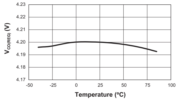
Constant Regulated Output Voltage vs. Temperature (AAT3681A, AAT3681A-1/-2/-4; R SET = 8.06kΩ)
