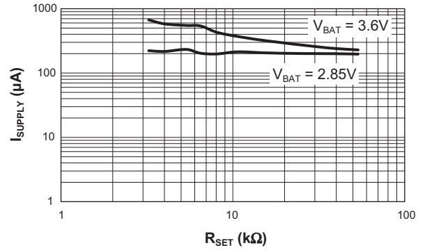
Operating Supply Current vs. R SET (V IN = 5V)
